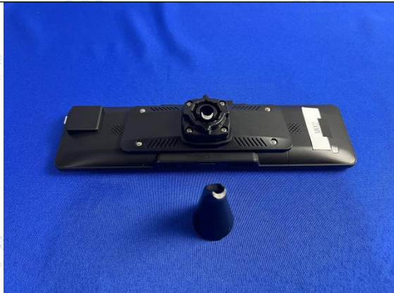
Fig.6 Appearance inspection after test (The front impact bracket has fractured.)
