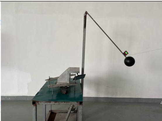
Fig.5 Test setup
