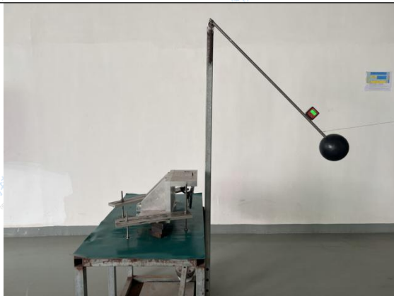
Fig.4 Test setup
