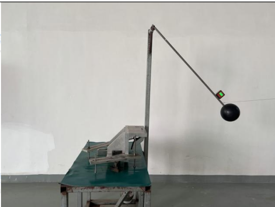
Fig.5 Test setup
