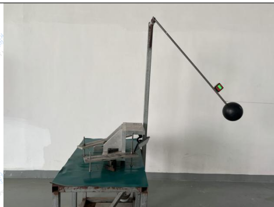
Fig.5 Test setup
