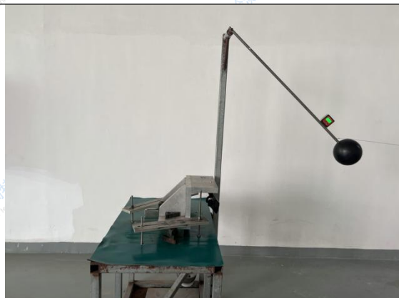
Fig.4 Test setup
